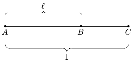
Figure 2. Appearance of the golden mean
