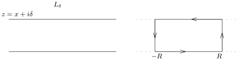
Figure 3. The line L_\delta and the contour \gamma_R
